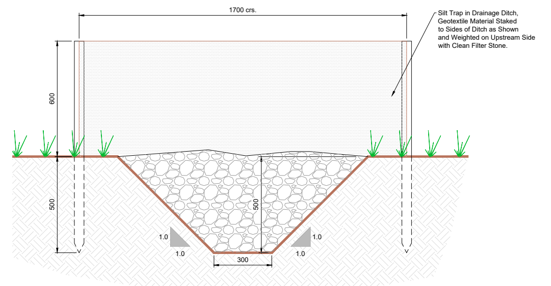
SILT TRAP IN DRAINAGE DITCH SECTION
