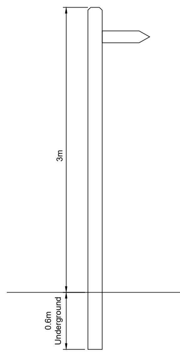
Fingerpost Sign
