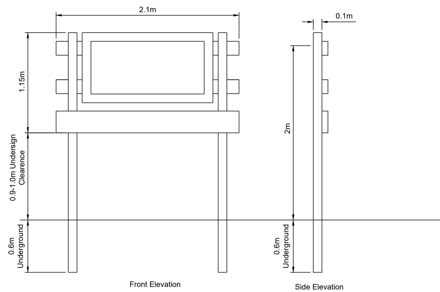
Threshold Sign
